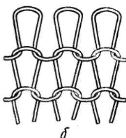
1-yuza; 2-iznanochnaya storona 60-rasm. Glad to'qimasi tuzilishi.
